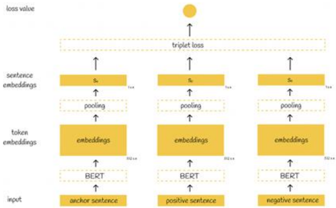
Figure 5.1: Sentence-BERT Diagram
